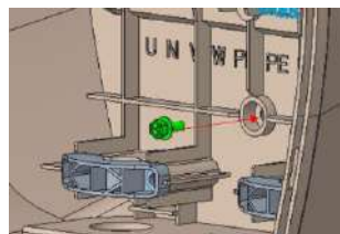
11. Fix lower screw
