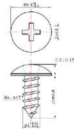
Phillips Pan Head Screw*2
