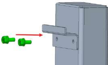
4. Install the bracket
