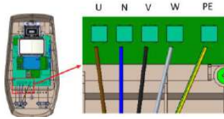
14. Connect AC inlet cable
