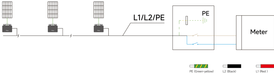
Wiring Diagram
